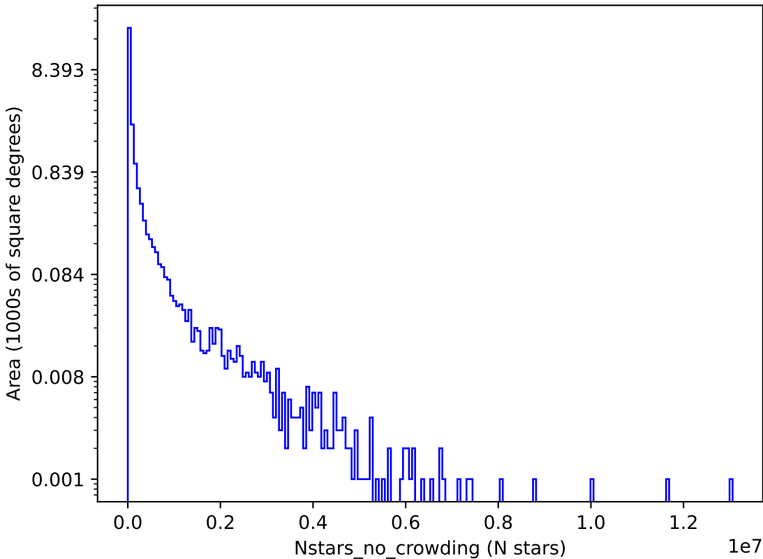
too_combined_s1.5_v3.4_10yrs g: Nstars_no_crowding
