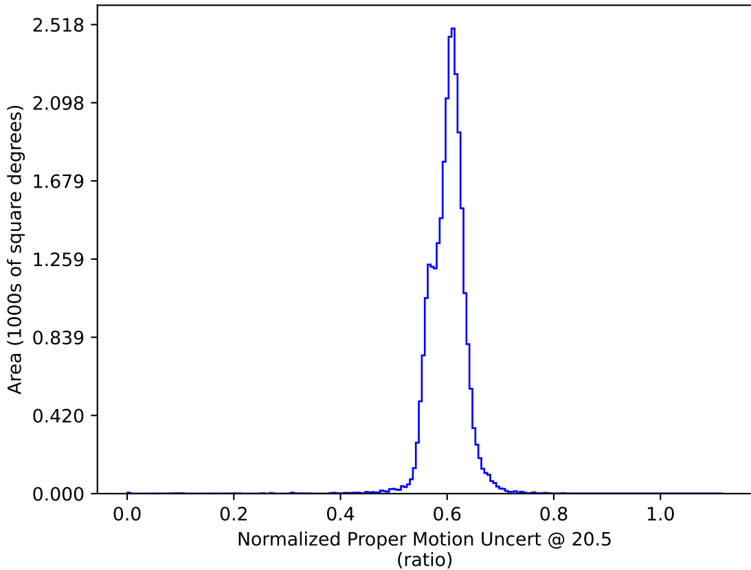
too_combined_s1.5_v3.4_10yrs : Normalized Proper Motion Uncert @ 20.5
