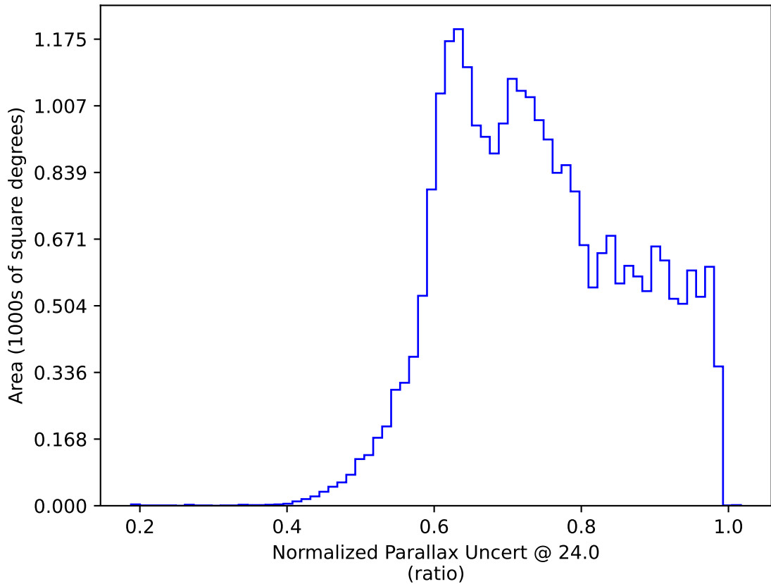
too_combined_s1.5_v3.4_10yrs : Normalized Parallax Uncert @ 24.0
