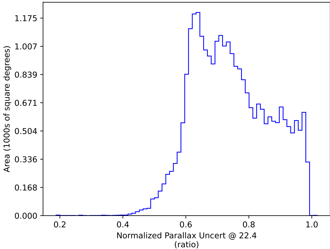
too_combined_s1.5_v3.4_10yrs : Normalized Parallax Uncert @ 22.4
