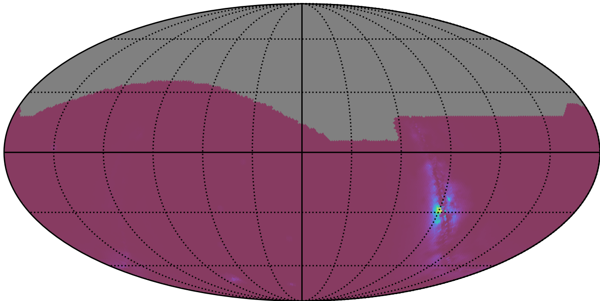
too_combined_s1.5_v3.4_10yrs : NlcPoints
