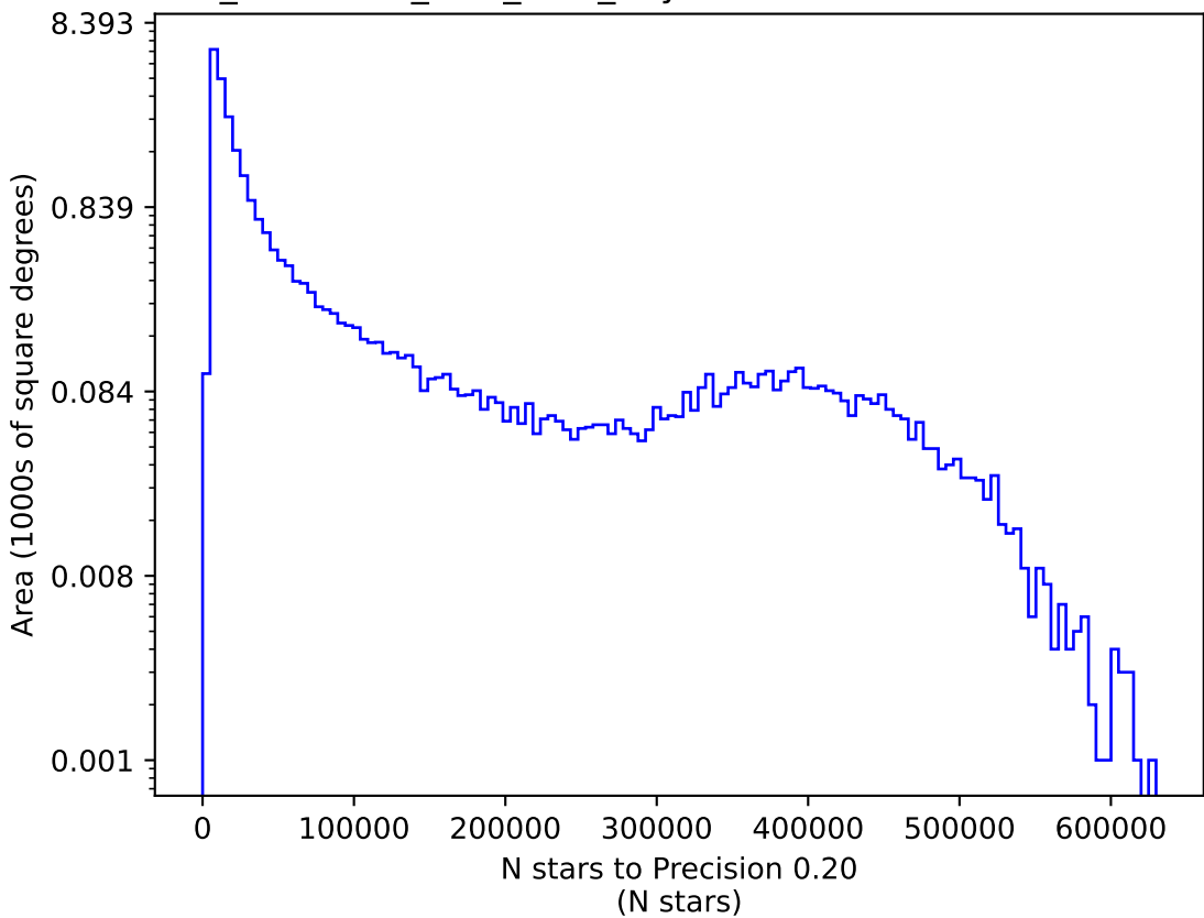
too_combined_s1.5_v3.4_10yrs z: N stars to Precision 0.20
