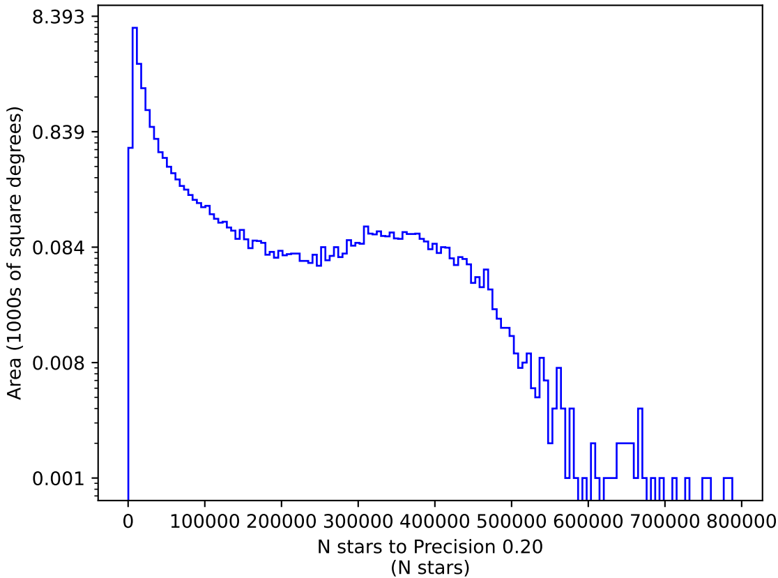
too_combined_s1.5_v3.4_10yrs y: N stars to Precision 0.20
