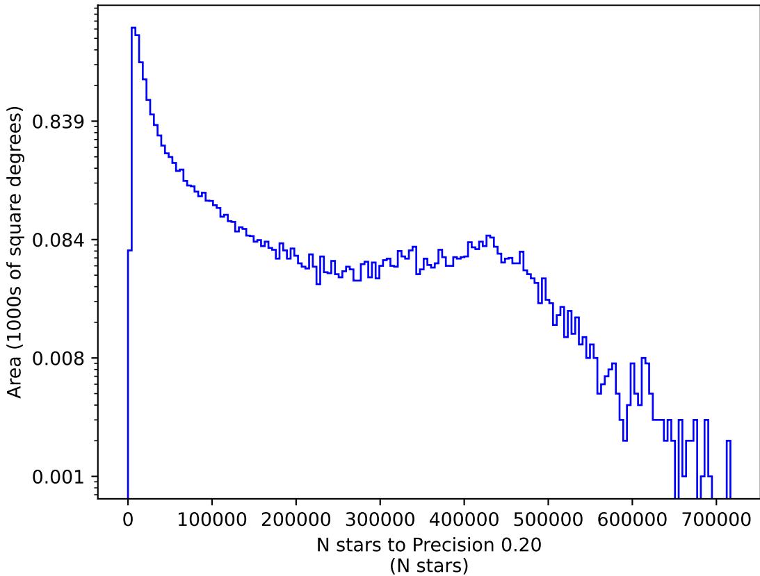
too_combined_s1.5_v3.4_10yrs r: N stars to Precision 0.20
