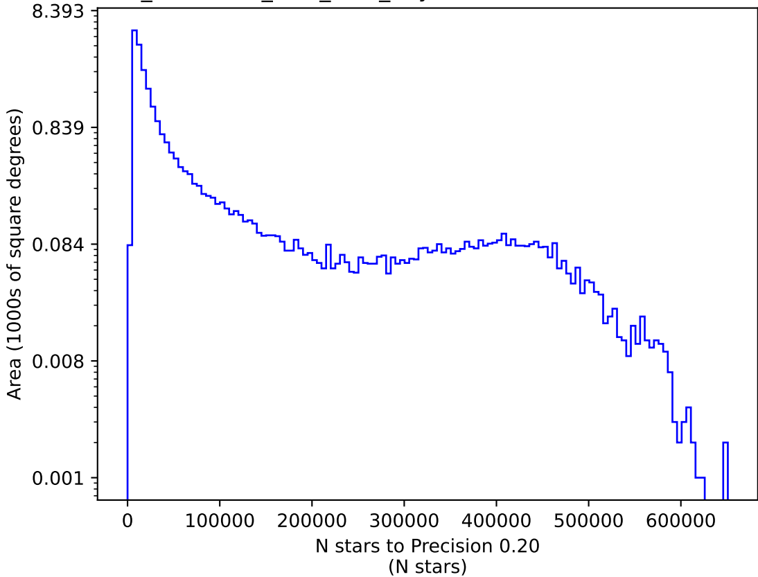
too_combined_s1.5_v3.4_10yrs i: N stars to Precision 0.20
