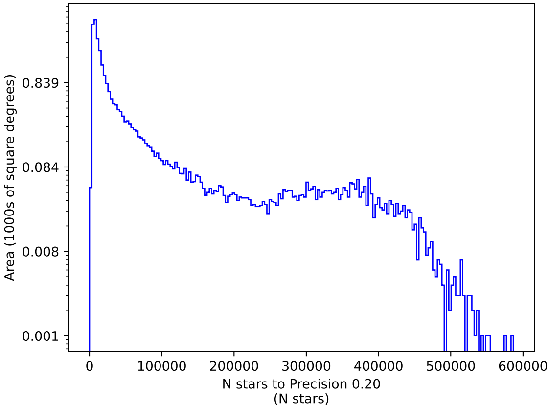
too_combined_s1.5_v3.4_10yrs g: N stars to Precision 0.20
