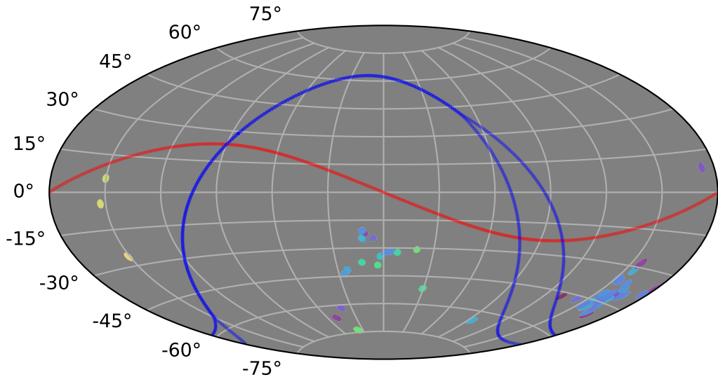
too_combined_s1.5_v3.4_10yrs gi: LVDwarfs
