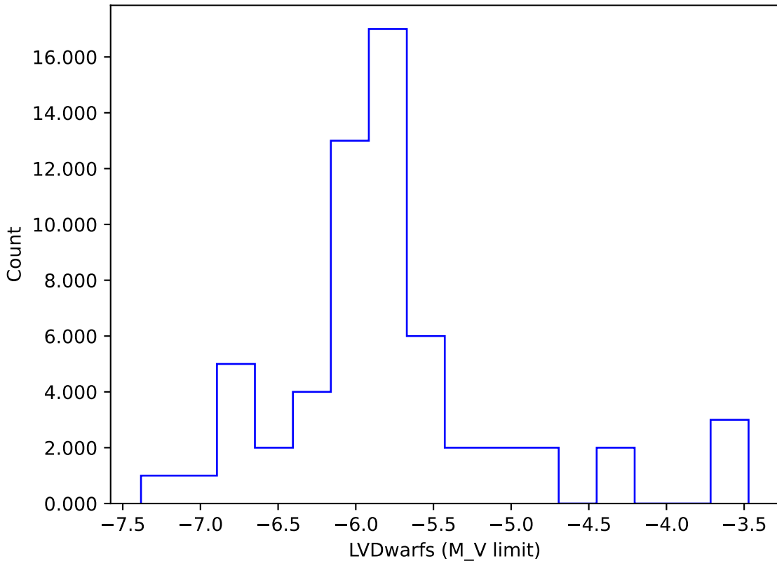
too_combined_s1.5_v3.4_10yrs gi: LVDwarfs
