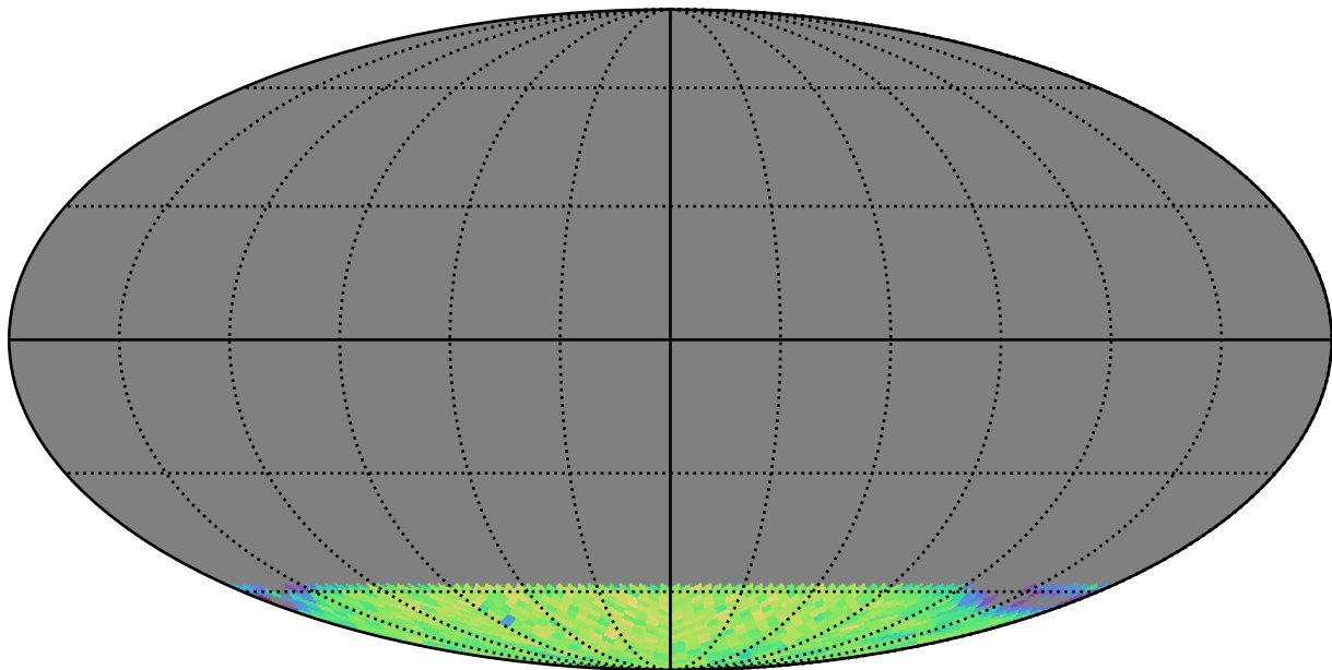
too_combined_s1.5_v3.4_10yrs gi SCP: LVDwarfs
