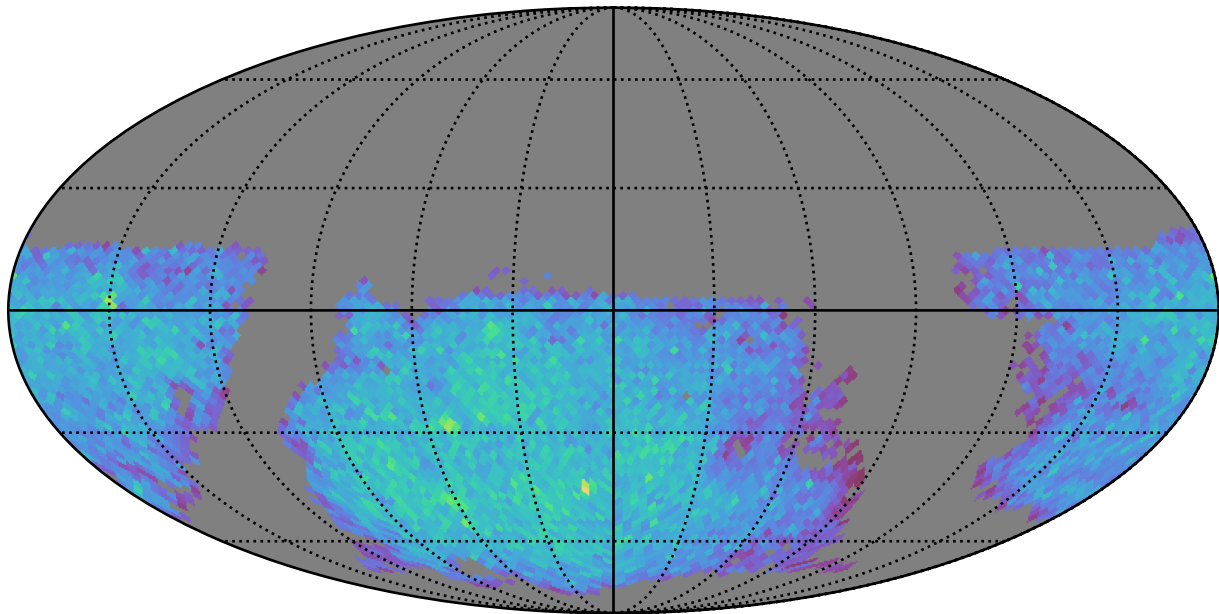
too_combined_s1.5_v3.4_10yrs gi: LVDwarfs
