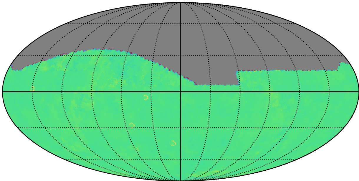
too_combined_s1.5_v3.4_10yrs z: Kuiper rotTelPos
