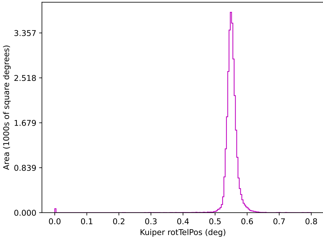
too_combined_s1.5_v3.4_10yrs z: Kuiper rotTelPos
