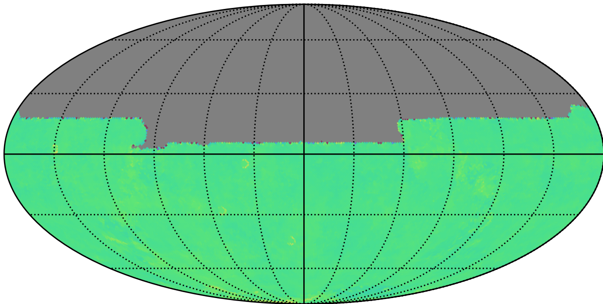
too_combined_s1.5_v3.4_10yrs y: Kuiper rotTelPos
