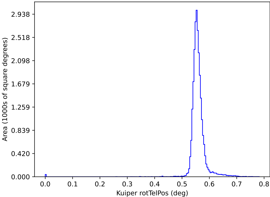
too_combined_s1.5_v3.4_10yrs y: Kuiper rotTelPos
