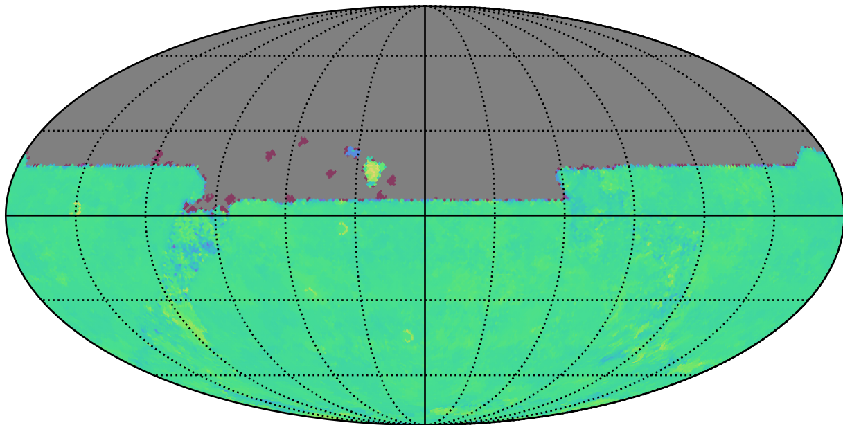
too_combined_s1.5_v3.4_10yrs u: Kuiper rotTelPos
