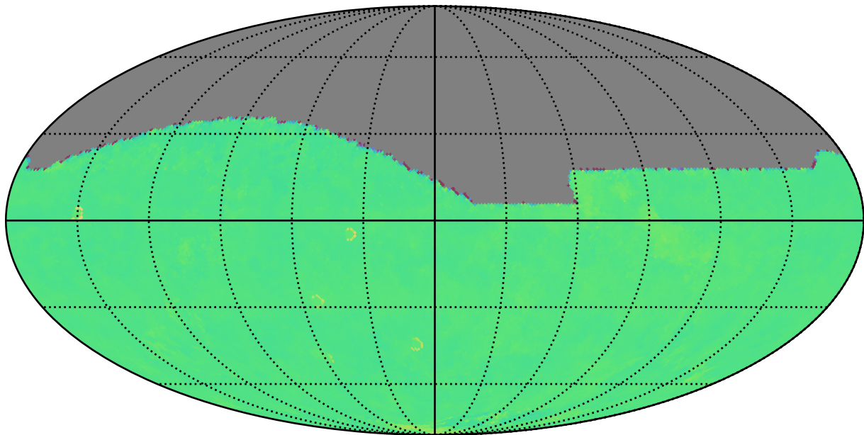
too_combined_s1.5_v3.4_10yrs r: Kuiper rotTelPos
