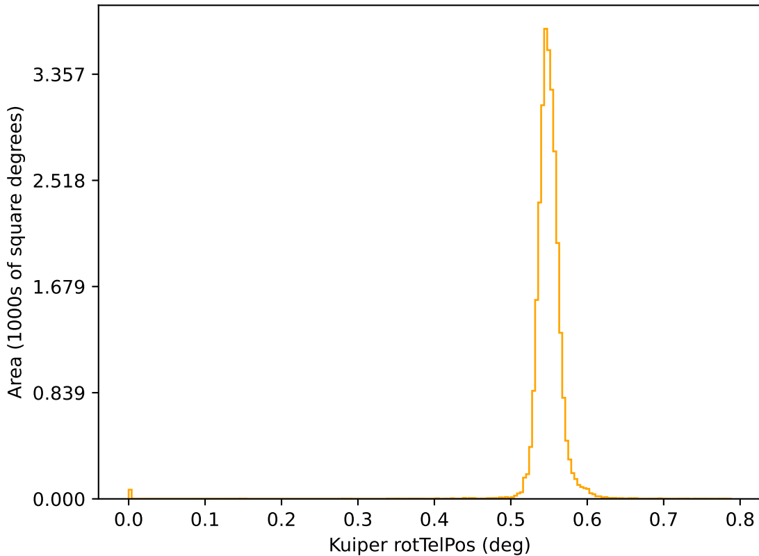
too_combined_s1.5_v3.4_10yrs r: Kuiper rotTelPos
