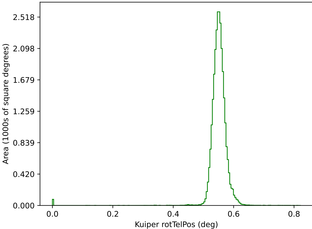
too_combined_s1.5_v3.4_10yrs g: Kuiper rotTelPos
