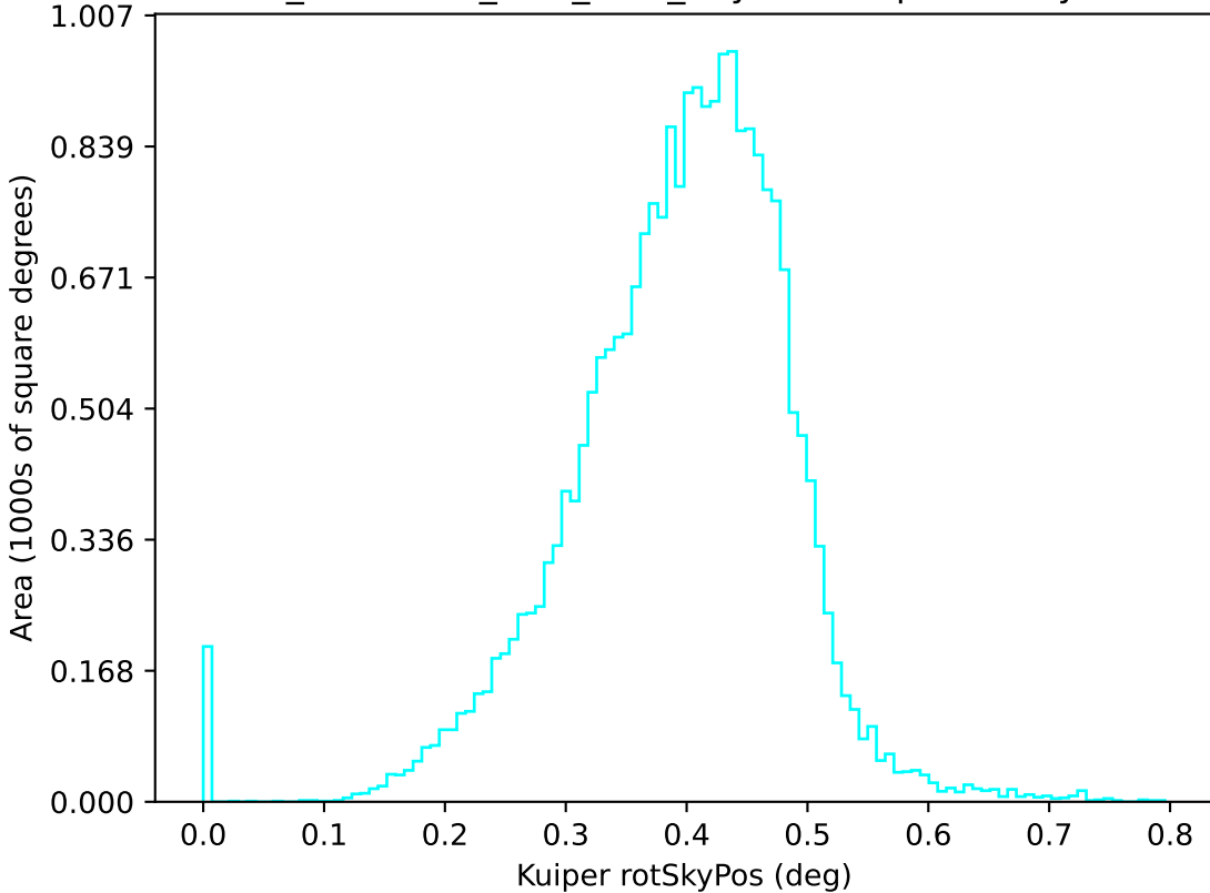
too_combined_s1.5_v3.4_10yrs u: Kuiper rotSkyPos
