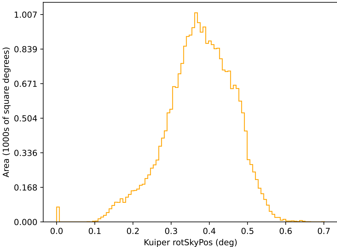
too_combined_s1.5_v3.4_10yrs r: Kuiper rotSkyPos
