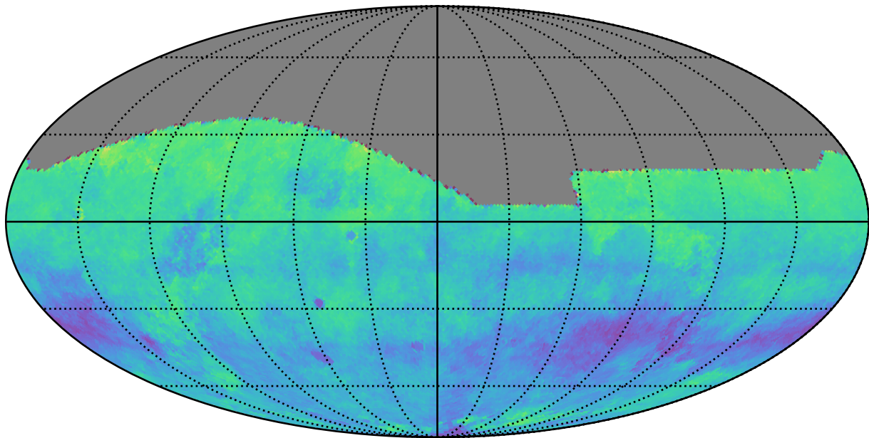
too_combined_s1.5_v3.4_10yrs i: Kuiper rotSkyPos
