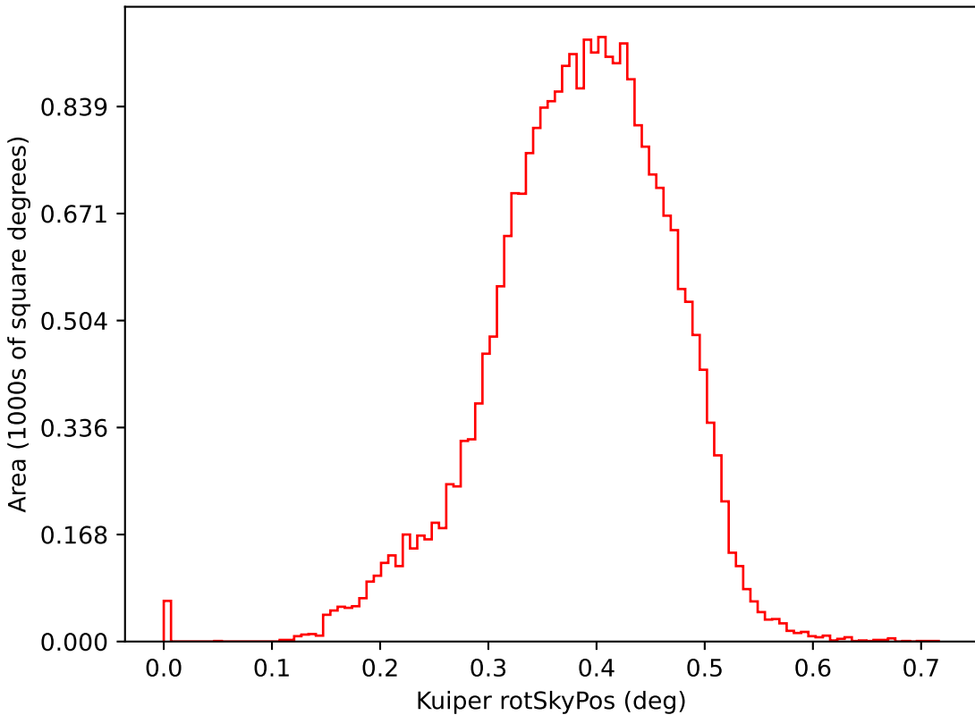
too_combined_s1.5_v3.4_10yrs i: Kuiper rotSkyPos
