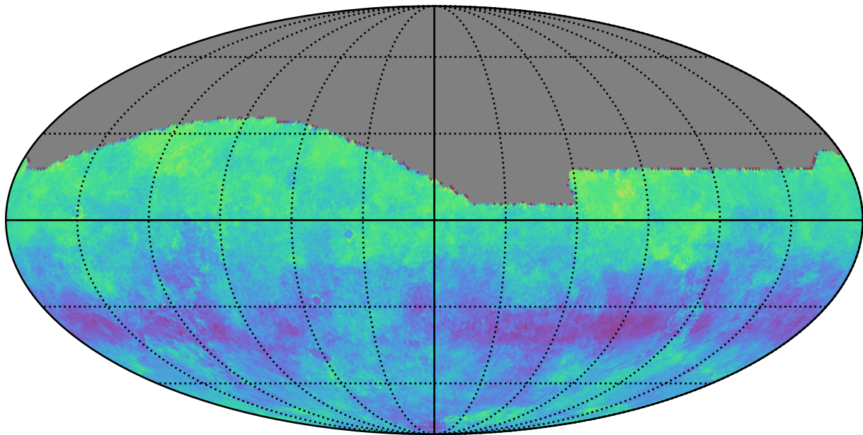
too_combined_s1.5_v3.4_10yrs g: Kuiper rotSkyPos
