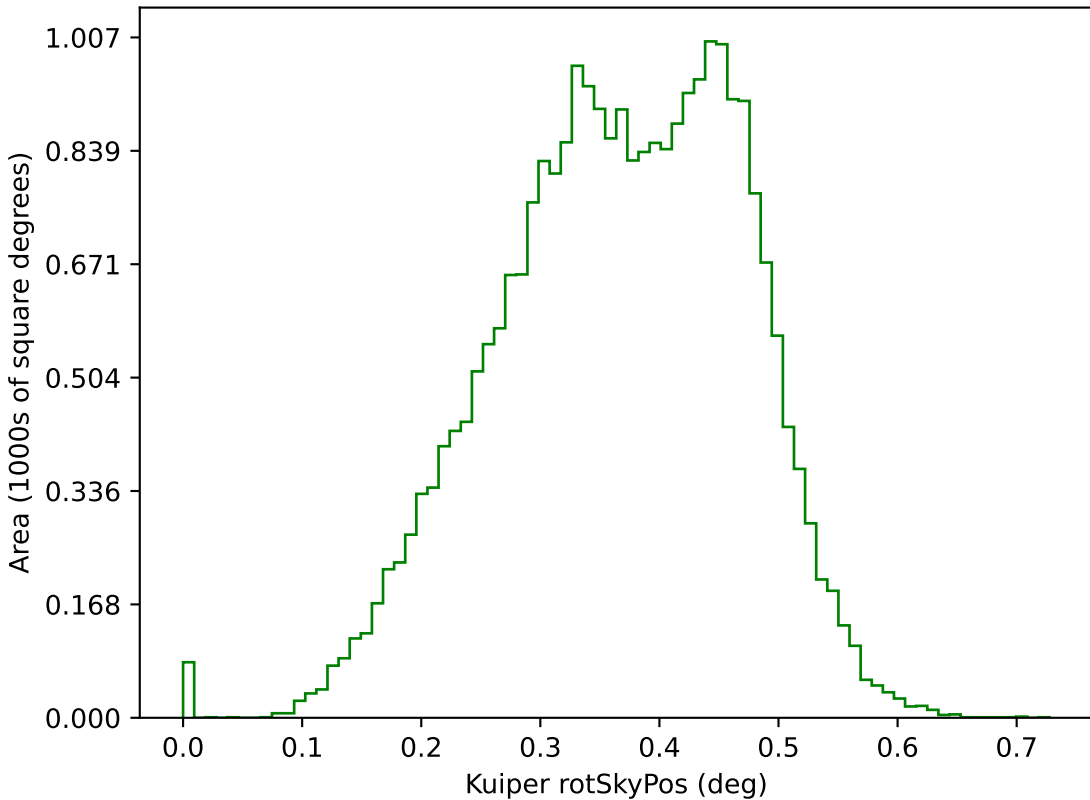
too_combined_s1.5_v3.4_10yrs g: Kuiper rotSkyPos
