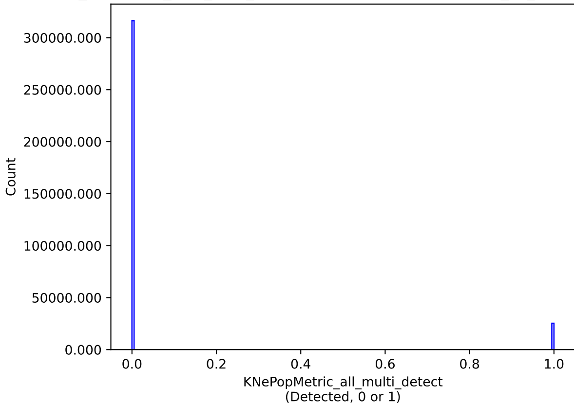
too_combined_s1.5_v3.4_10yrs all models: KNePopMetric_all_multi_detect
