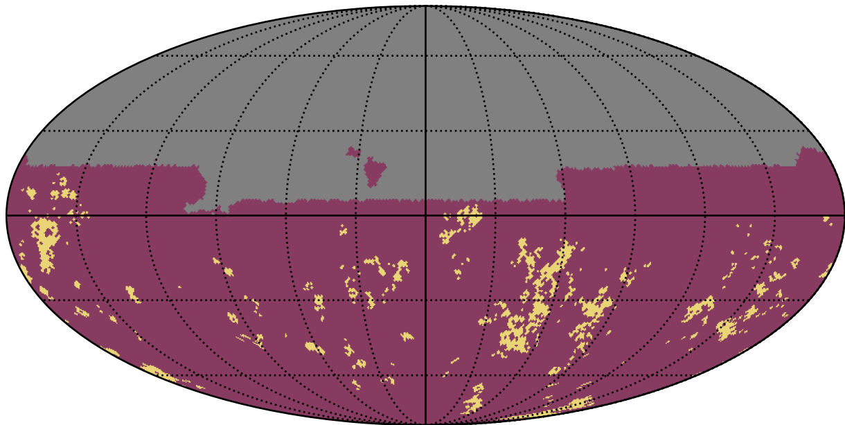
too_combined_s1.5_v3.4_10yrs u band: Gaps_7hr
