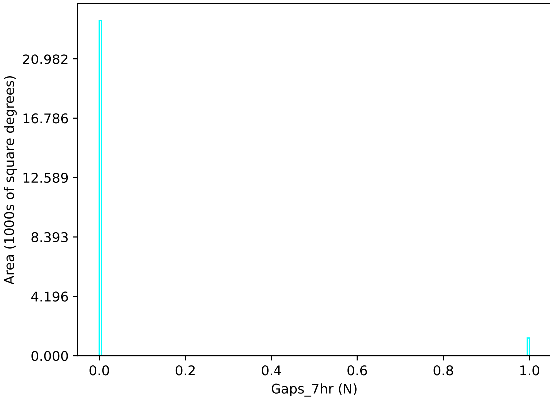
too_combined_s1.5_v3.4_10yrs u band: Gaps_7hr
