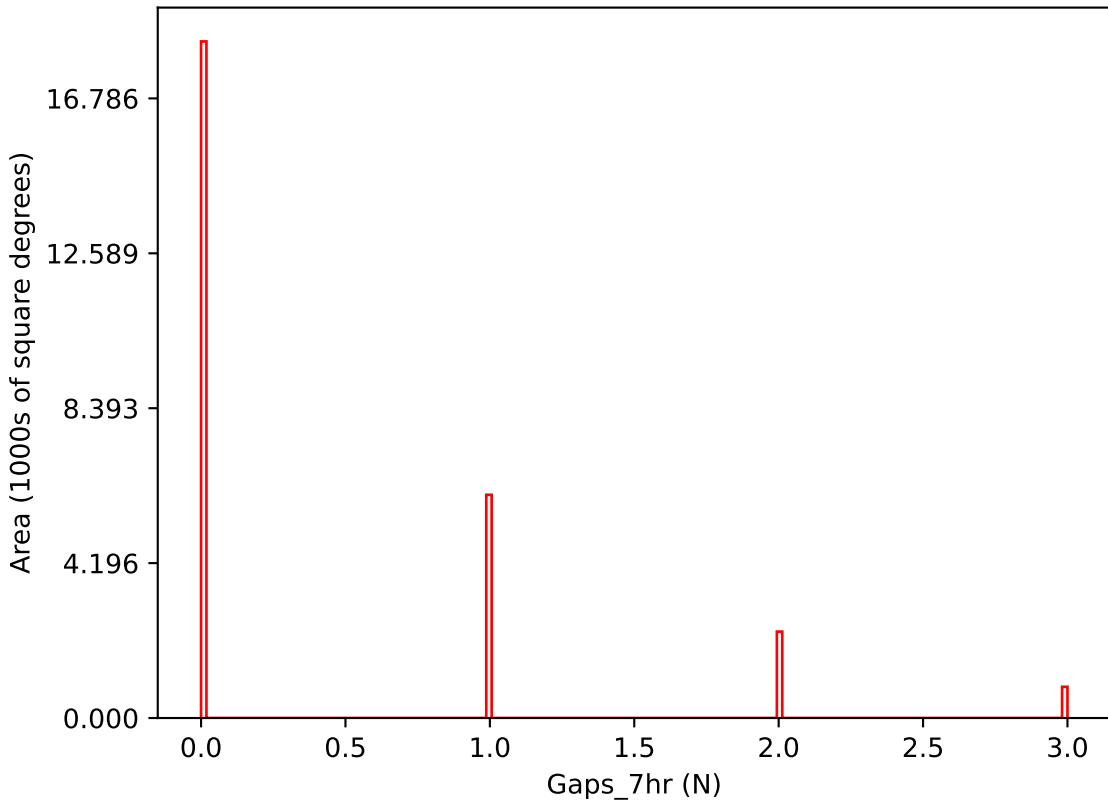
too_combined_s1.5_v3.4_10yrs i band: Gaps_7hr
