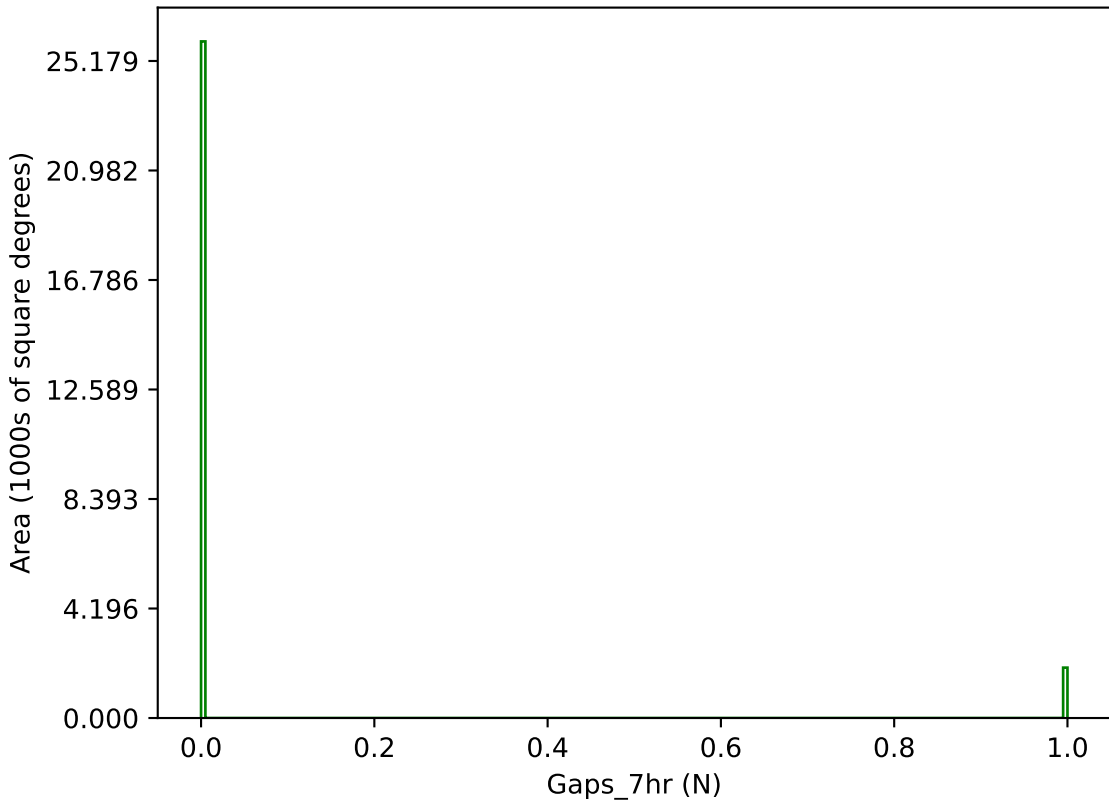
too_combined_s1.5_v3.4_10yrs g band: Gaps_7hr
