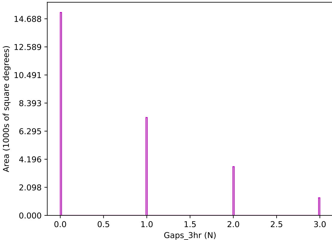
too_combined_s1.5_v3.4_10yrs z band: Gaps_3hr
