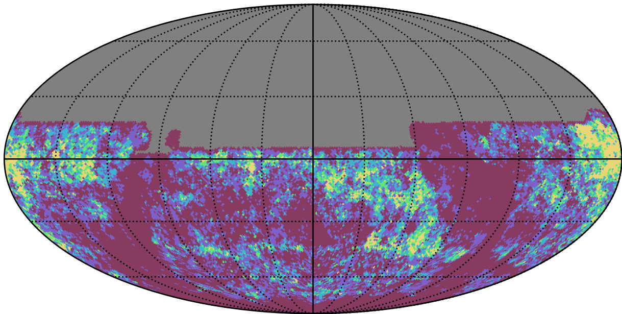
too_combined_s1.5_v3.4_10yrs y band: Gaps_3hr
