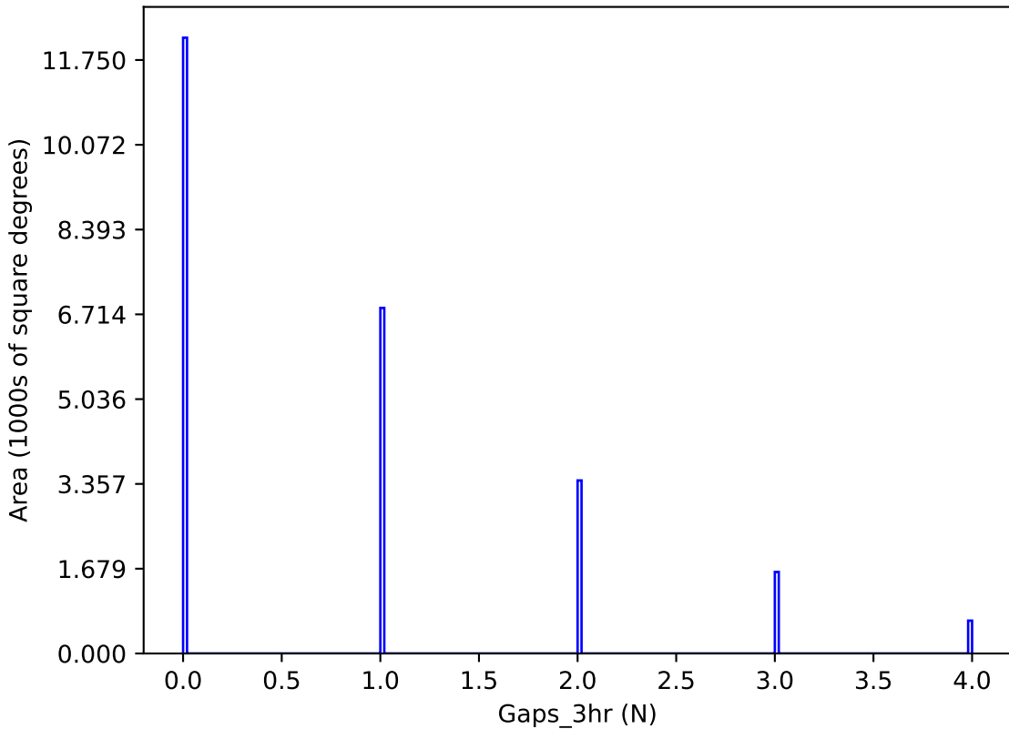
too_combined_s1.5_v3.4_10yrs y band: Gaps_3hr
