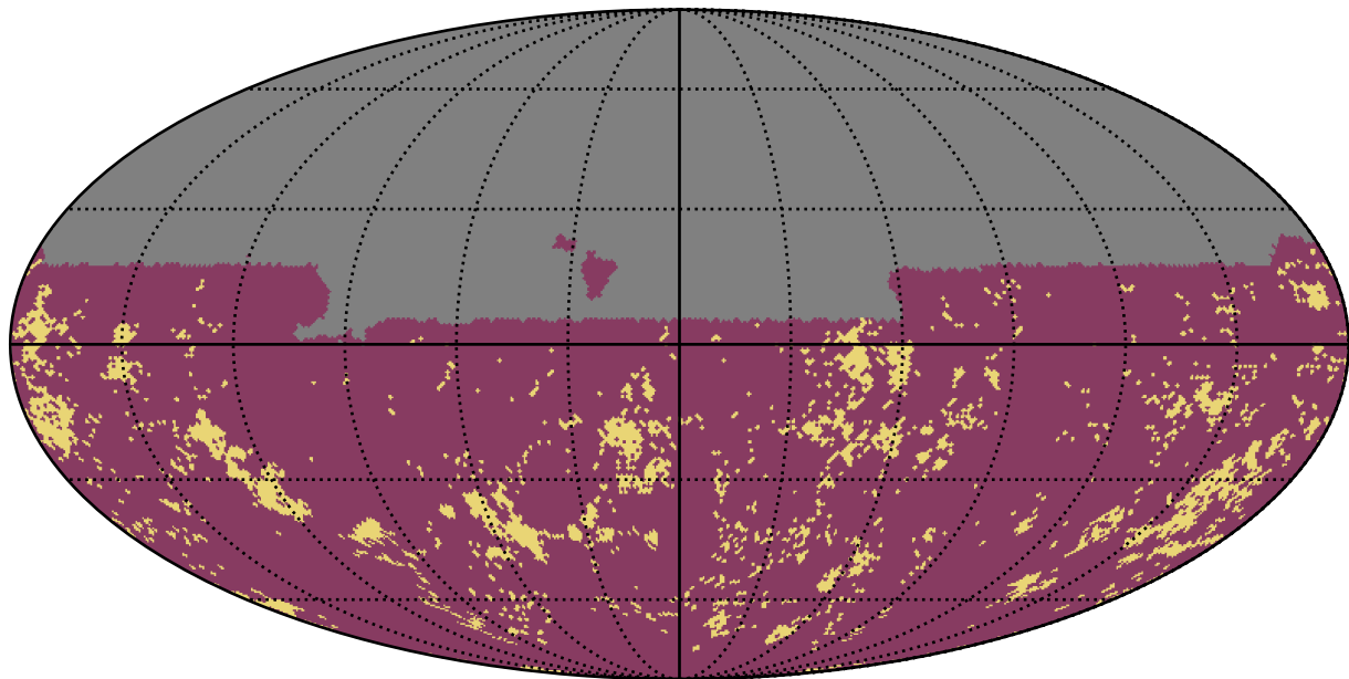
too_combined_s1.5_v3.4_10yrs u band: Gaps_3hr
