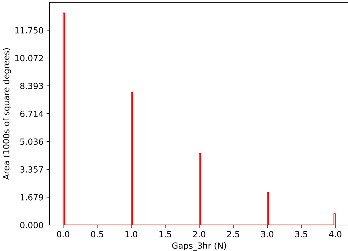
too_combined_s1.5_v3.4_10yrs i band: Gaps_3hr
