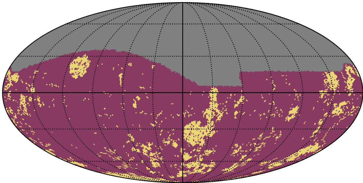
too_combined_s1.5_v3.4_10yrs g band: Gaps_3hr
