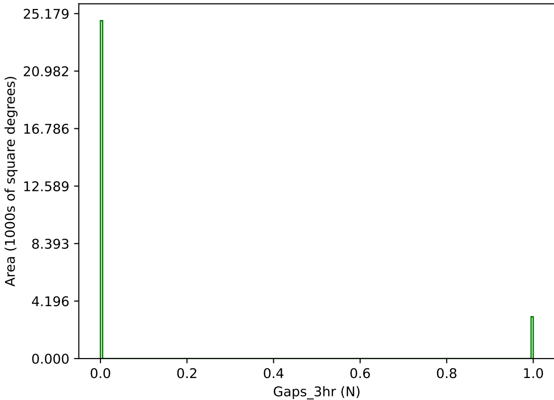
too_combined_s1.5_v3.4_10yrs g band: Gaps_3hr
