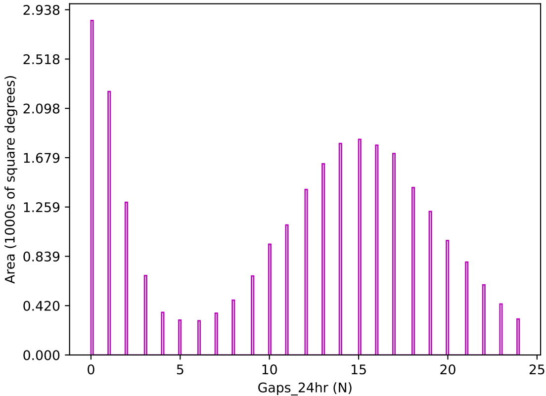
too_combined_s1.5_v3.4_10yrs z band: Gaps_24hr
