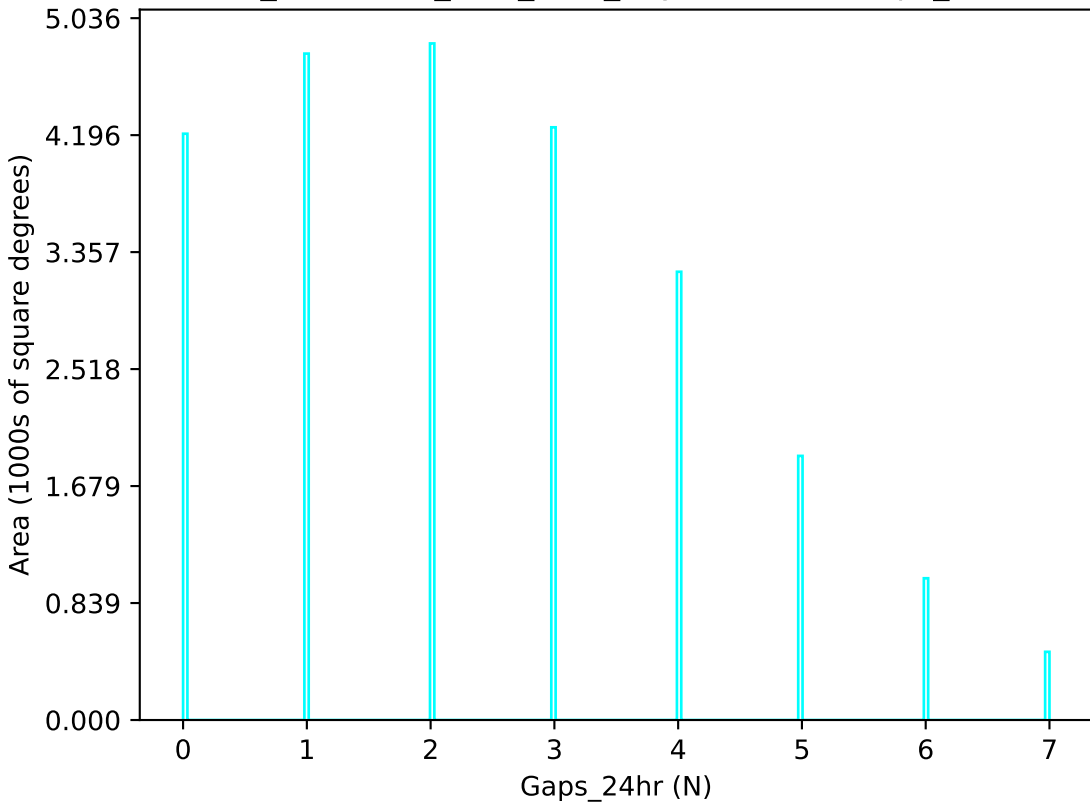
too_combined_s1.5_v3.4_10yrs u band: Gaps_24hr
