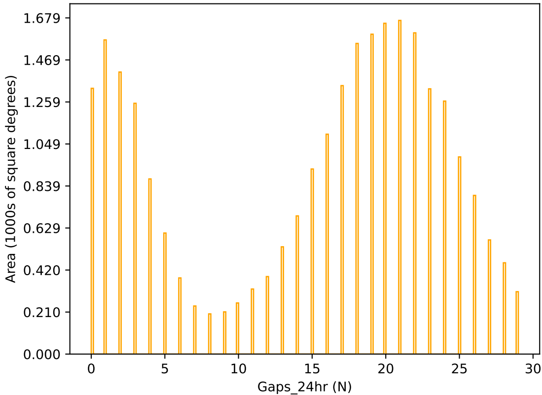
too_combined_s1.5_v3.4_10yrs r band: Gaps_24hr
