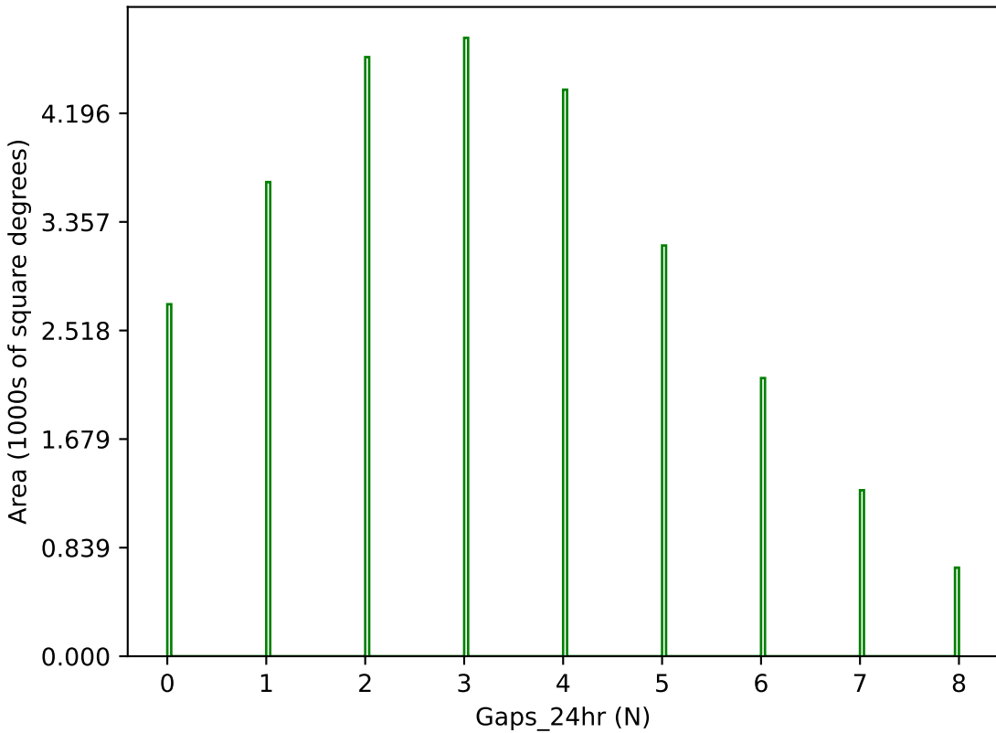
too_combined_s1.5_v3.4_10yrs g band: Gaps_24hr
