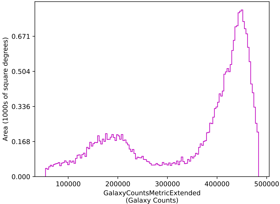
too_combined_s1.5_v3.4_10yrs z: GalaxyCountsMetricExtended
