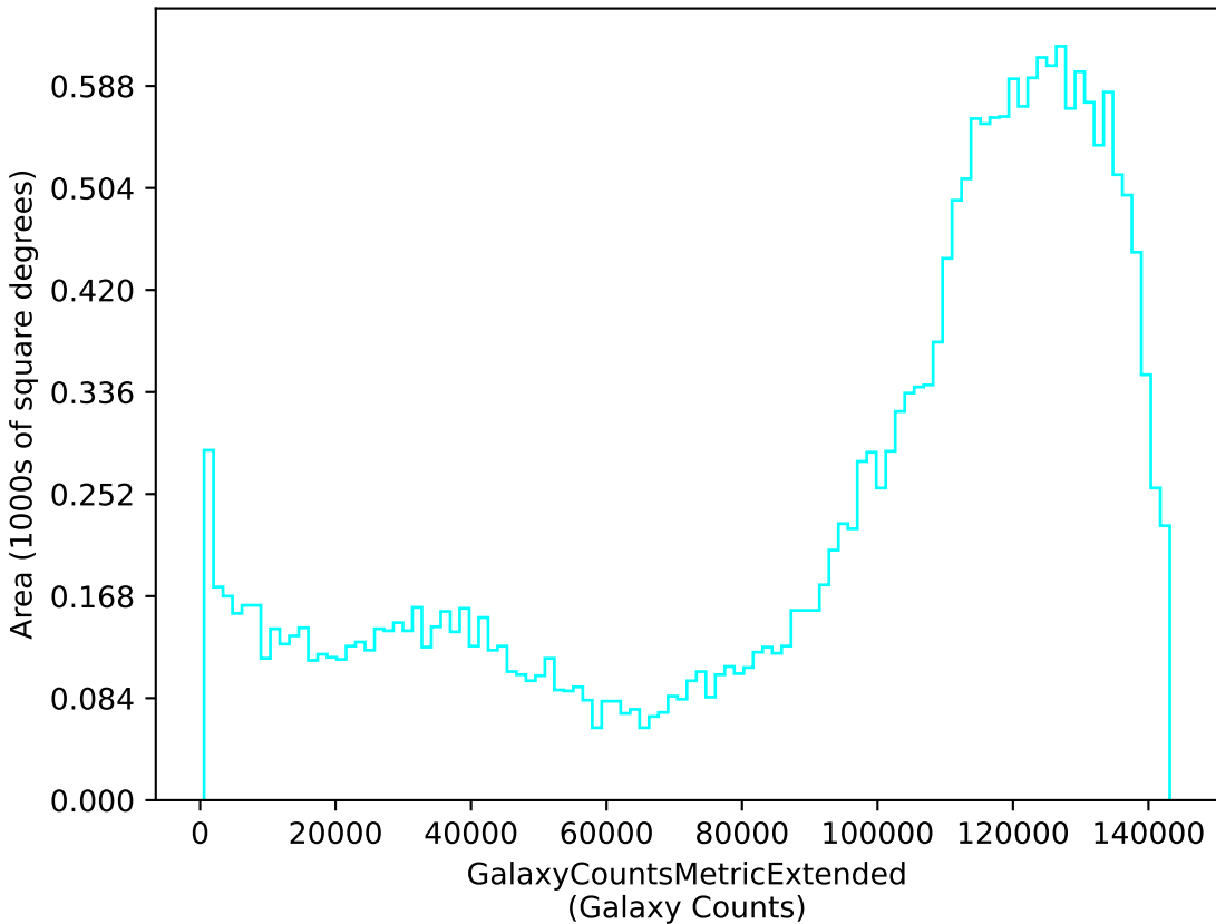
too_combined_s1.5_v3.4_10yrs u: GalaxyCountsMetricExtended
