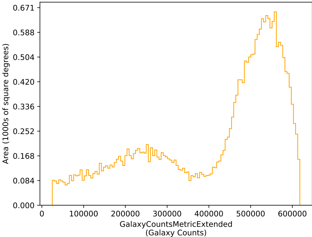
too_combined_s1.5_v3.4_10yrs r: GalaxyCountsMetricExtended
