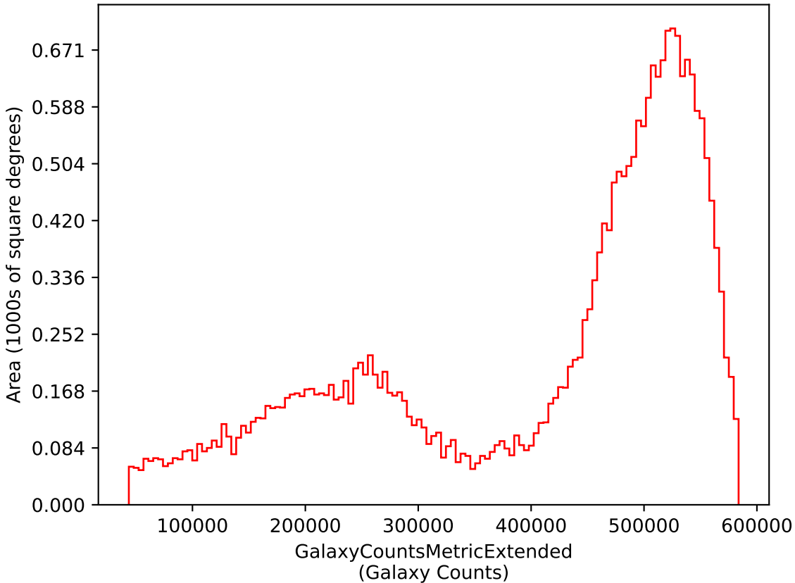
too_combined_s1.5_v3.4_10yrs i: GalaxyCountsMetricExtended
