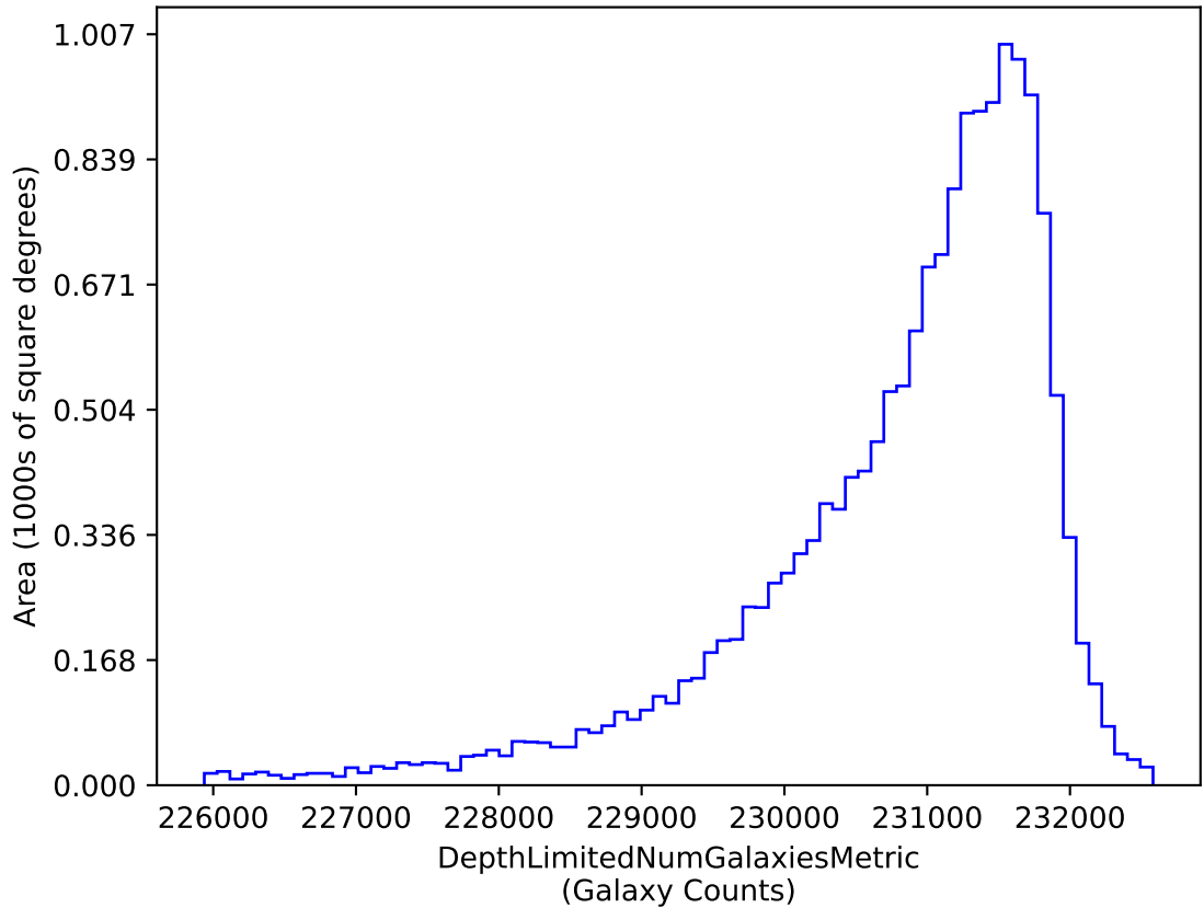
too_combined_s1.5_v3.4_10yrs i band galaxies non-DD: DepthLimitedNumGalaxiesMetric
