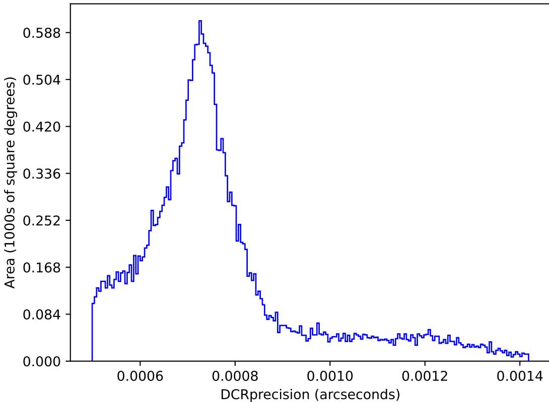
too_combined_s1.5_v3.4_10yrs : DCRprecision
